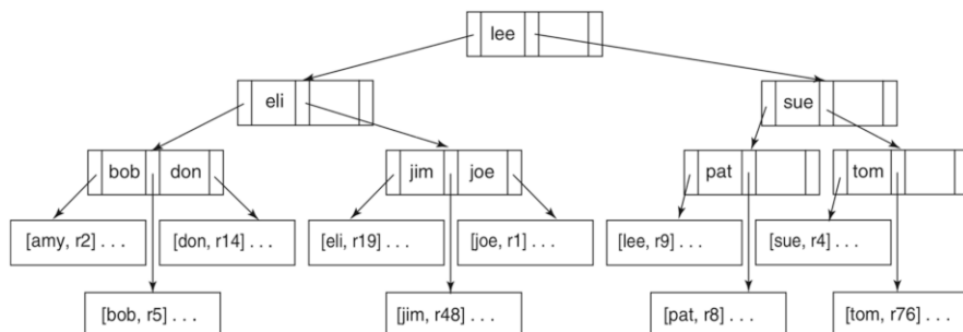
Fig. 12.18 Splitting the root of the B-tree
