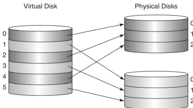
Fig. 3.3 Disk striping
