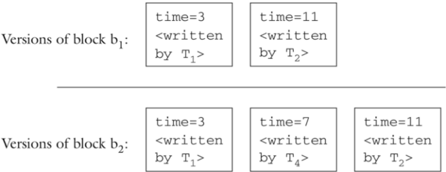
Fig. 5.24 Multiversion concurrency
