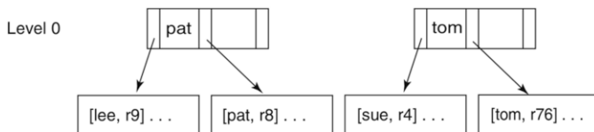
Fig. 12.17 Splitting a directory block
